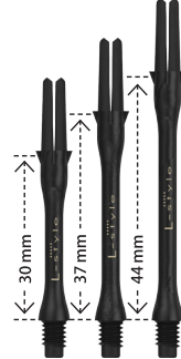
L-Shaft Lock Slim
